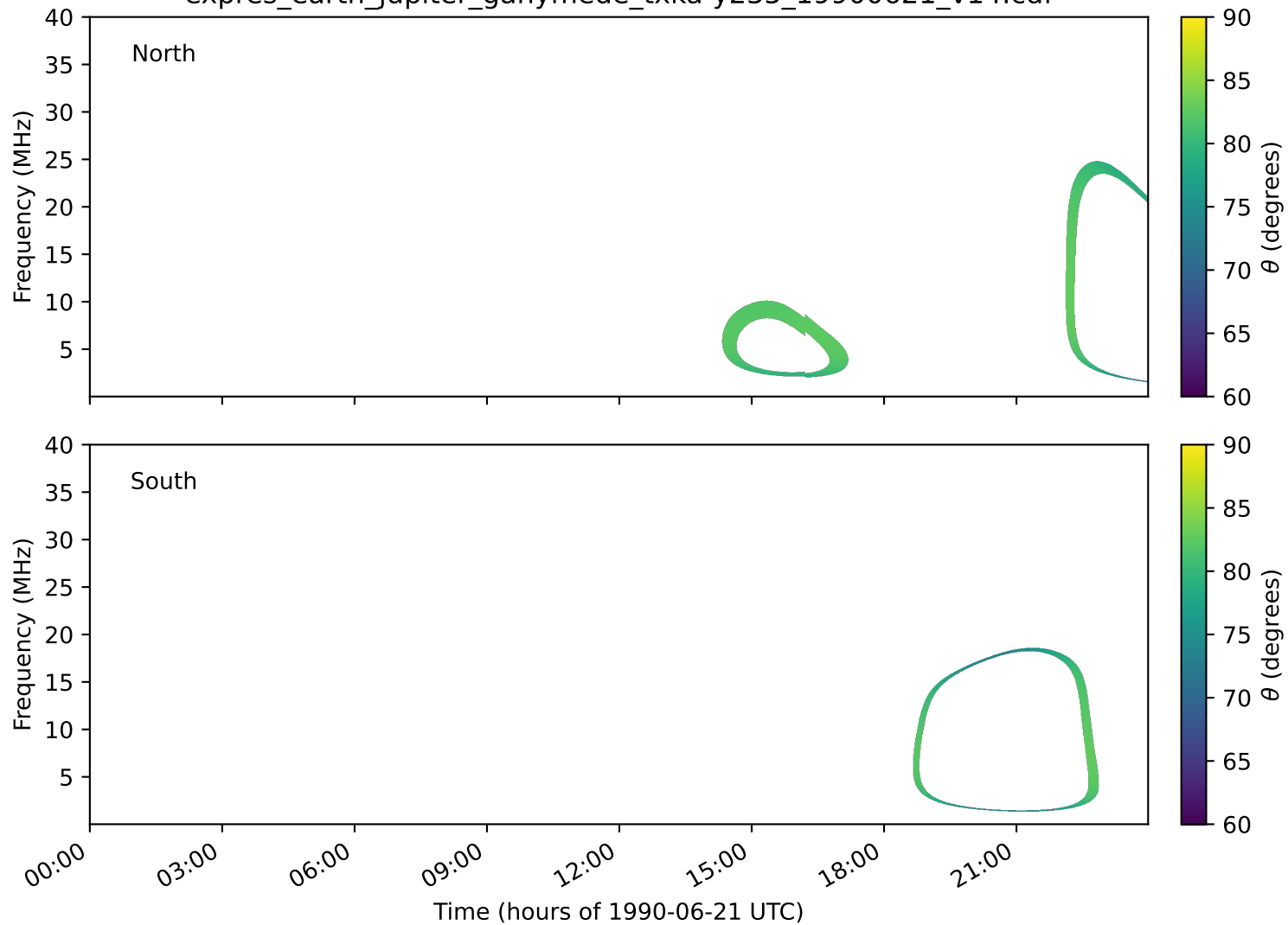
expres_earth_jupiter_ganymede_txka-y235_19900621_v14.cdf
