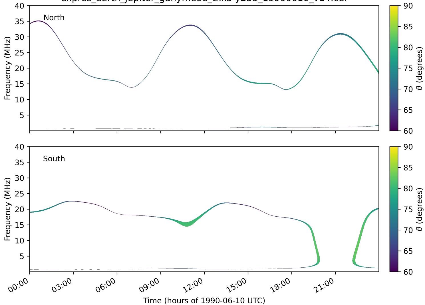
expres_earth_jupiter_ganymede_txka-y235_19900610_v14.cdf
