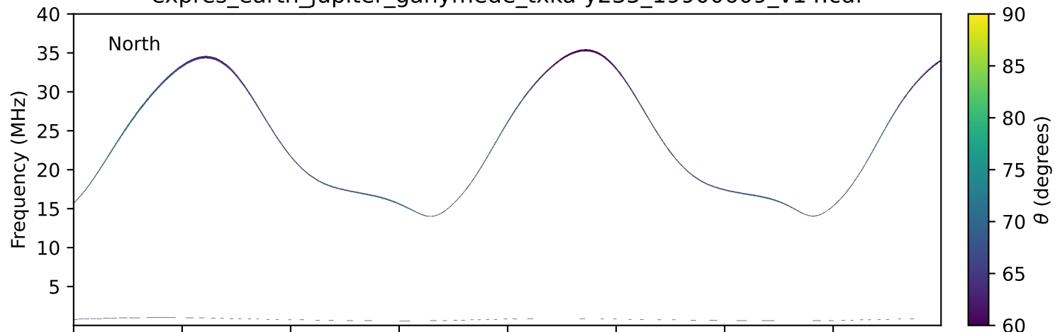
expres_earth_jupiter_ganymede_txka-y235_19900609_v14.cdf
