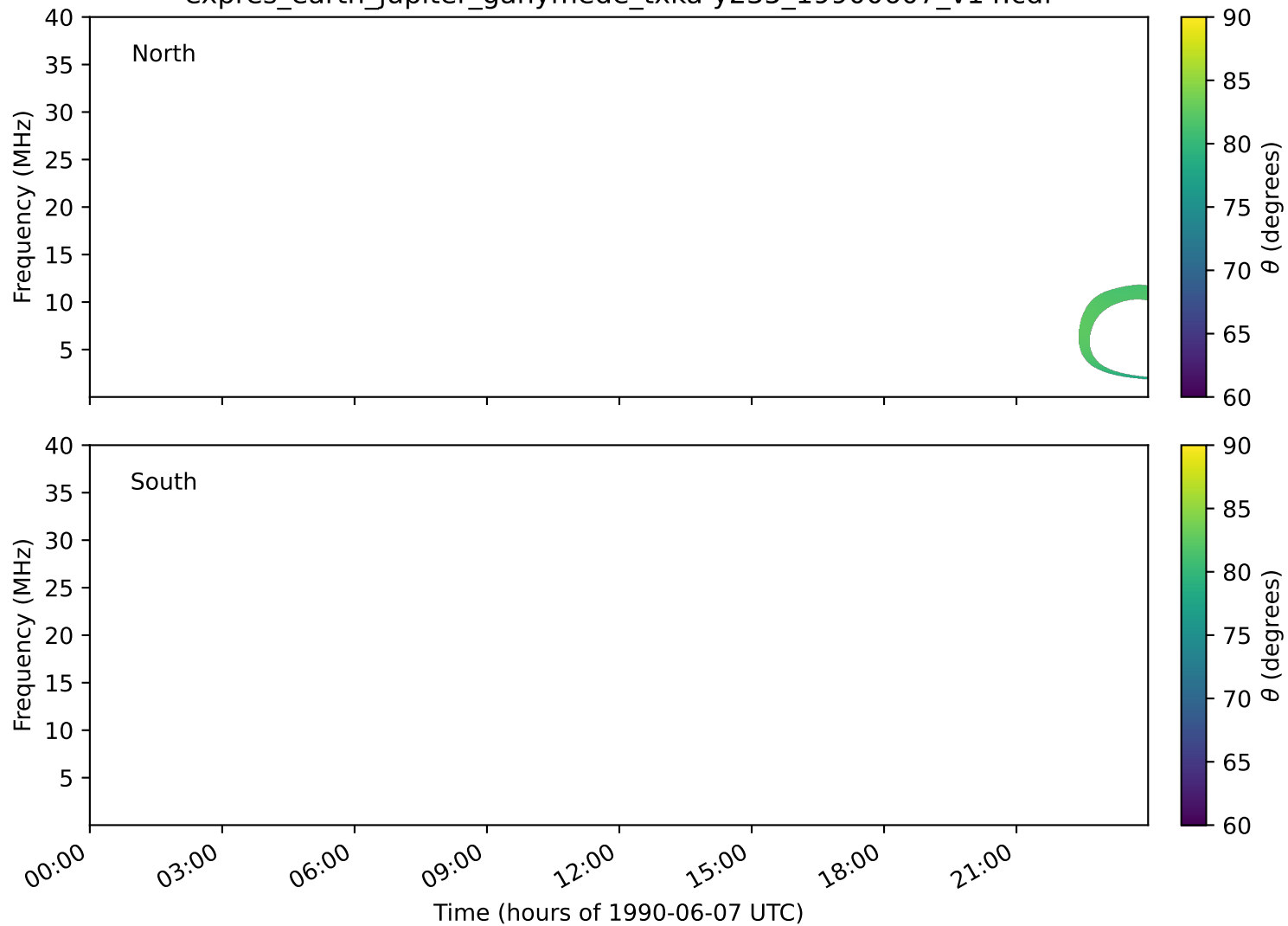
expres_earth_jupiter_ganymede_txka-y235_19900607_v14.cdf
