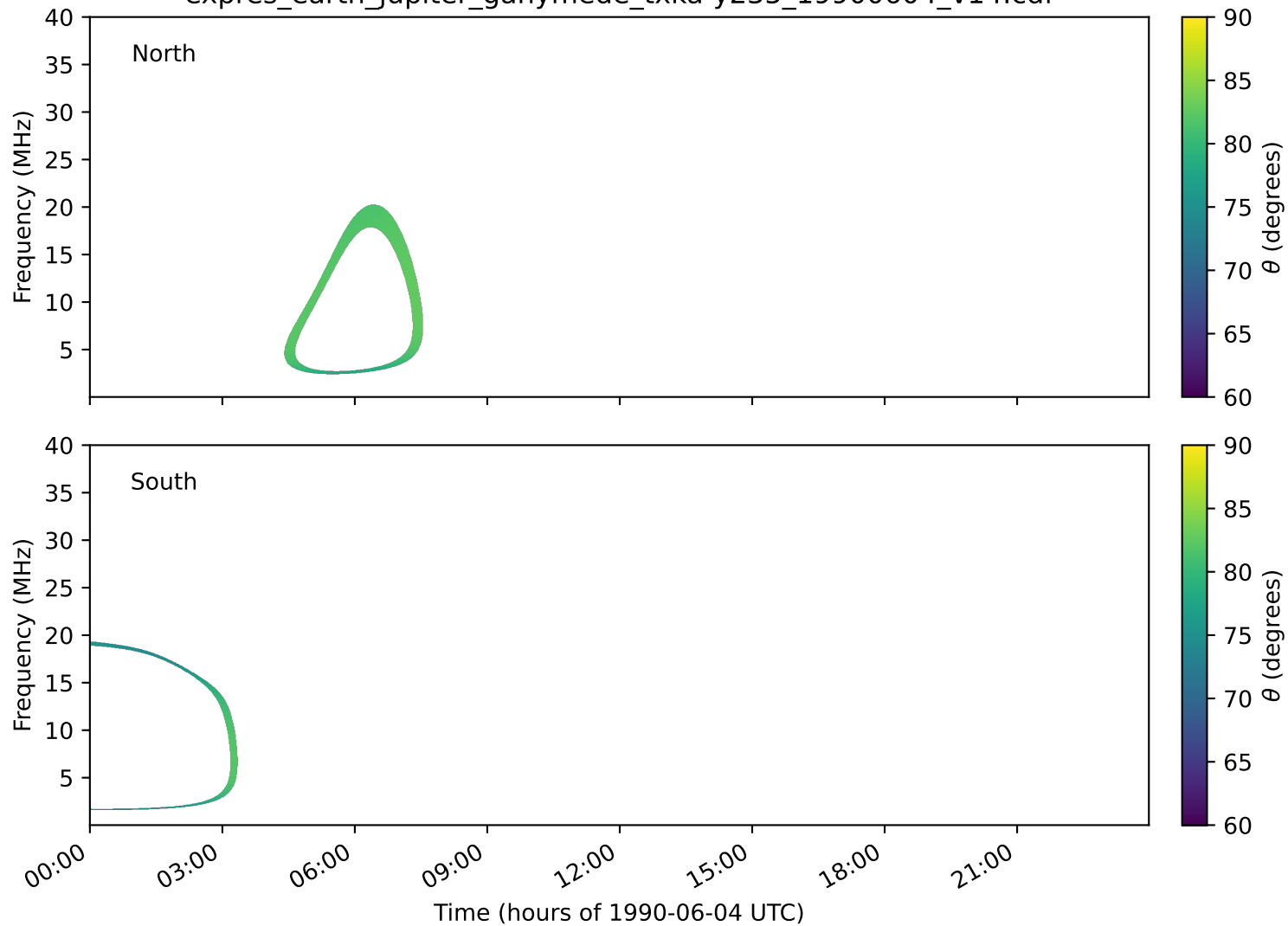
expres_earth_jupiter_ganymede_txka-y235_19900604_v14.cdf
