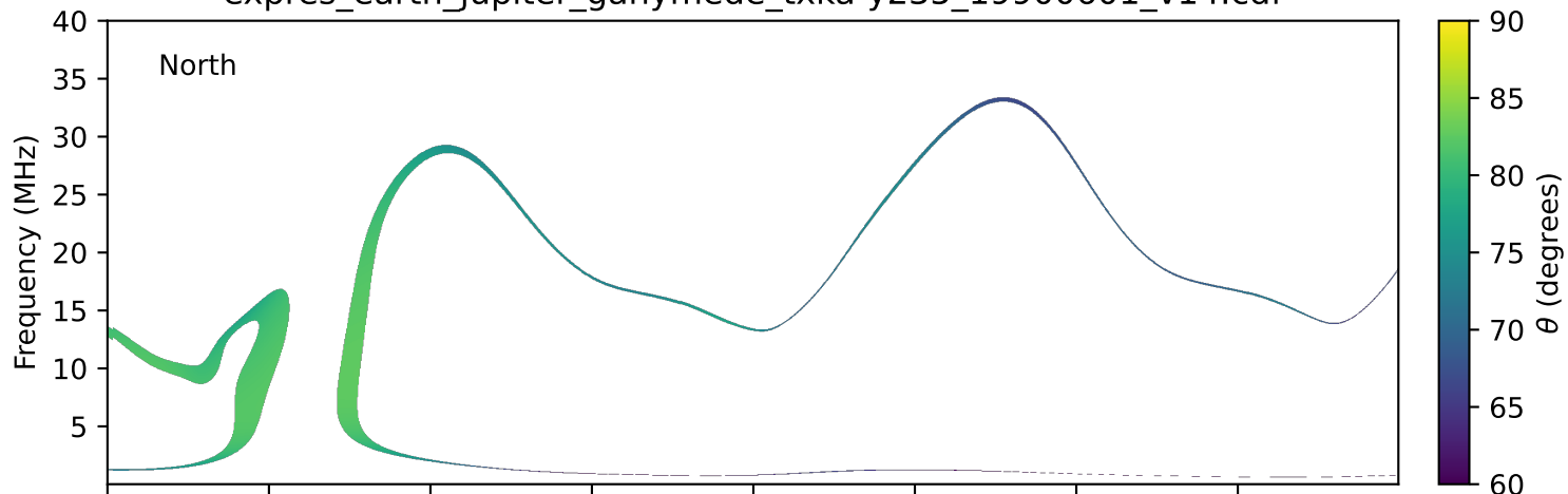
expres_earth_jupiter_ganymede_txka-y235_19900601_v14.cdf
