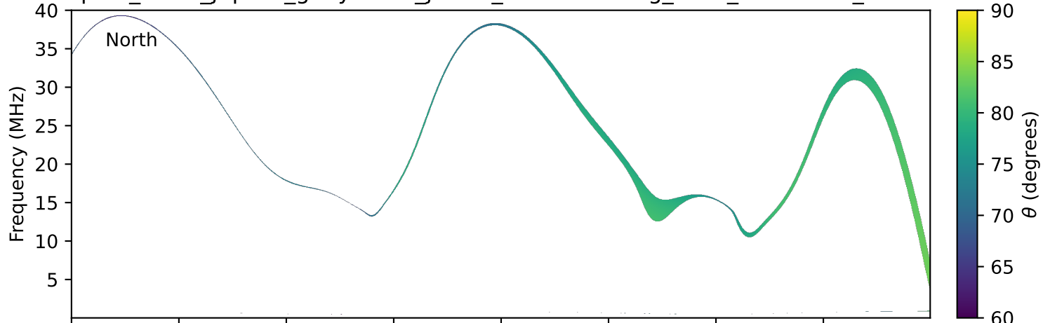
expres_earth_jupiter_ganymede_jrm09_lossc-wid1deg_3kev_19900617_v11.cdf
