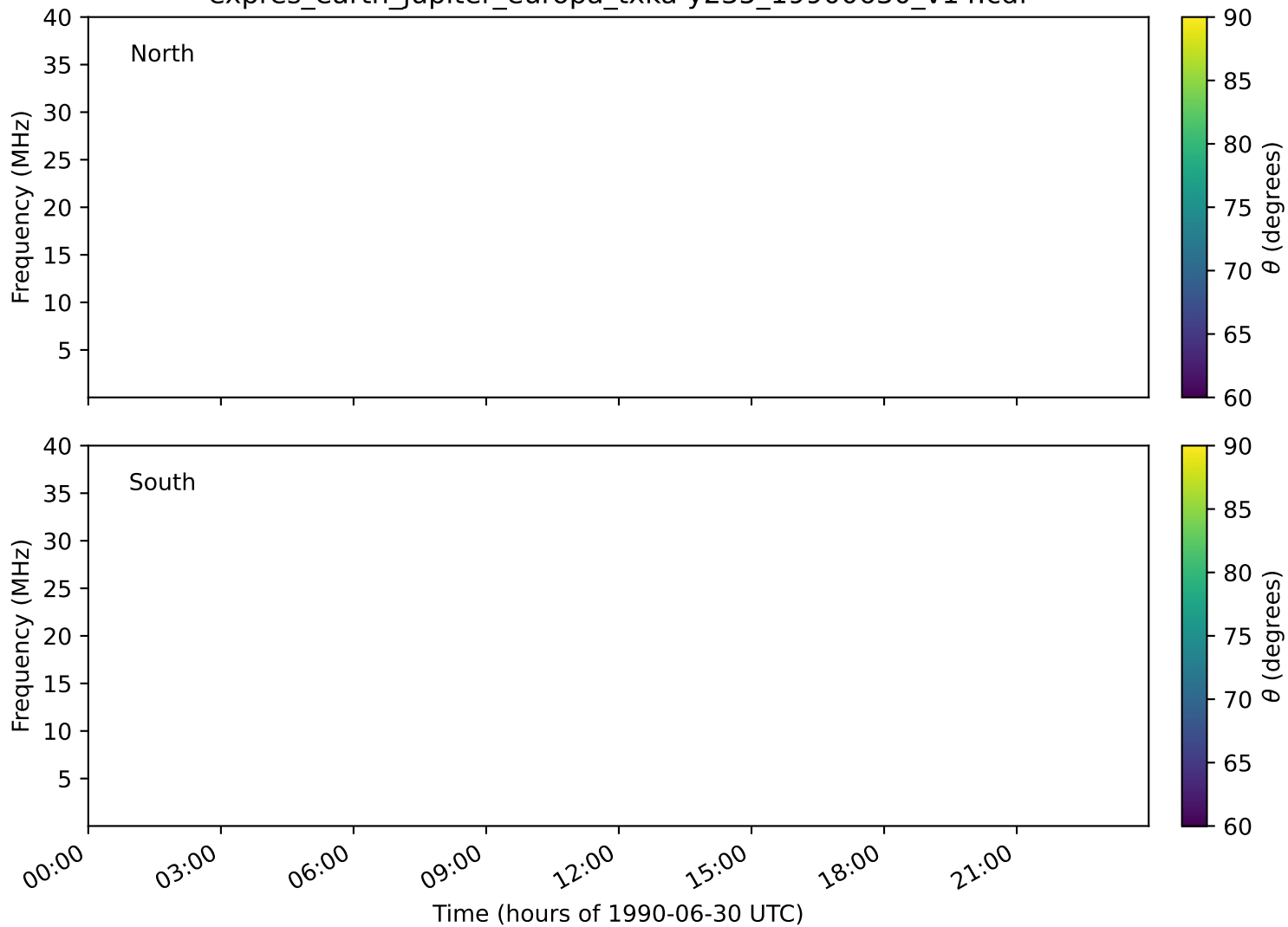
expres_earth_jupiter_europa_txka-y235_19900630_v14.cdf
