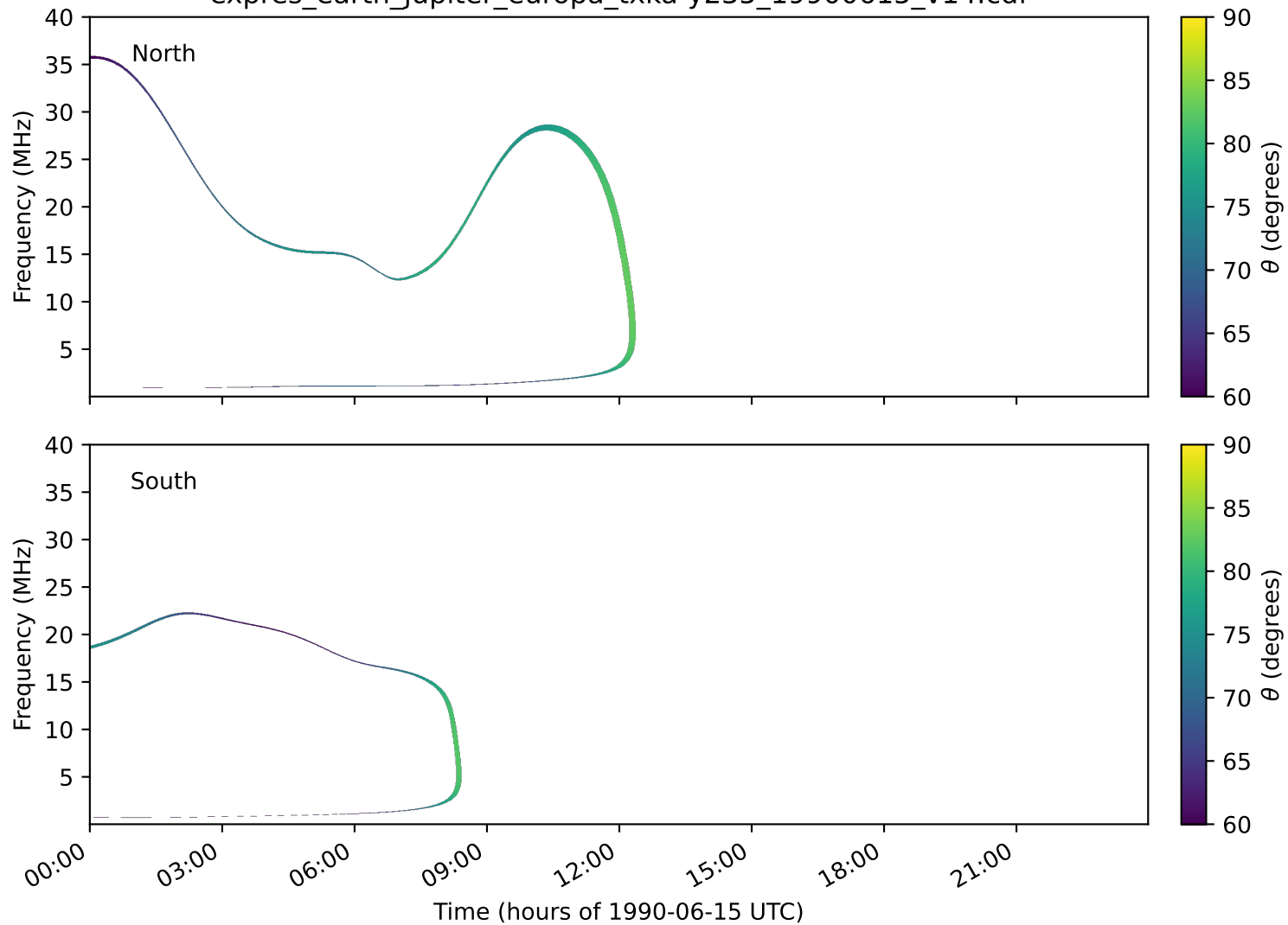
expres_earth_jupiter_europa_txka-y235_19900615_v14.cdf
