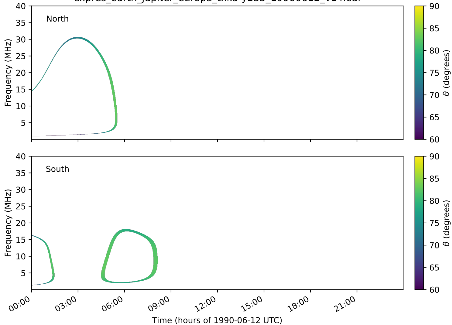
expres_earth_jupiter_europa_txka-y235_19900612_v14.cdf
