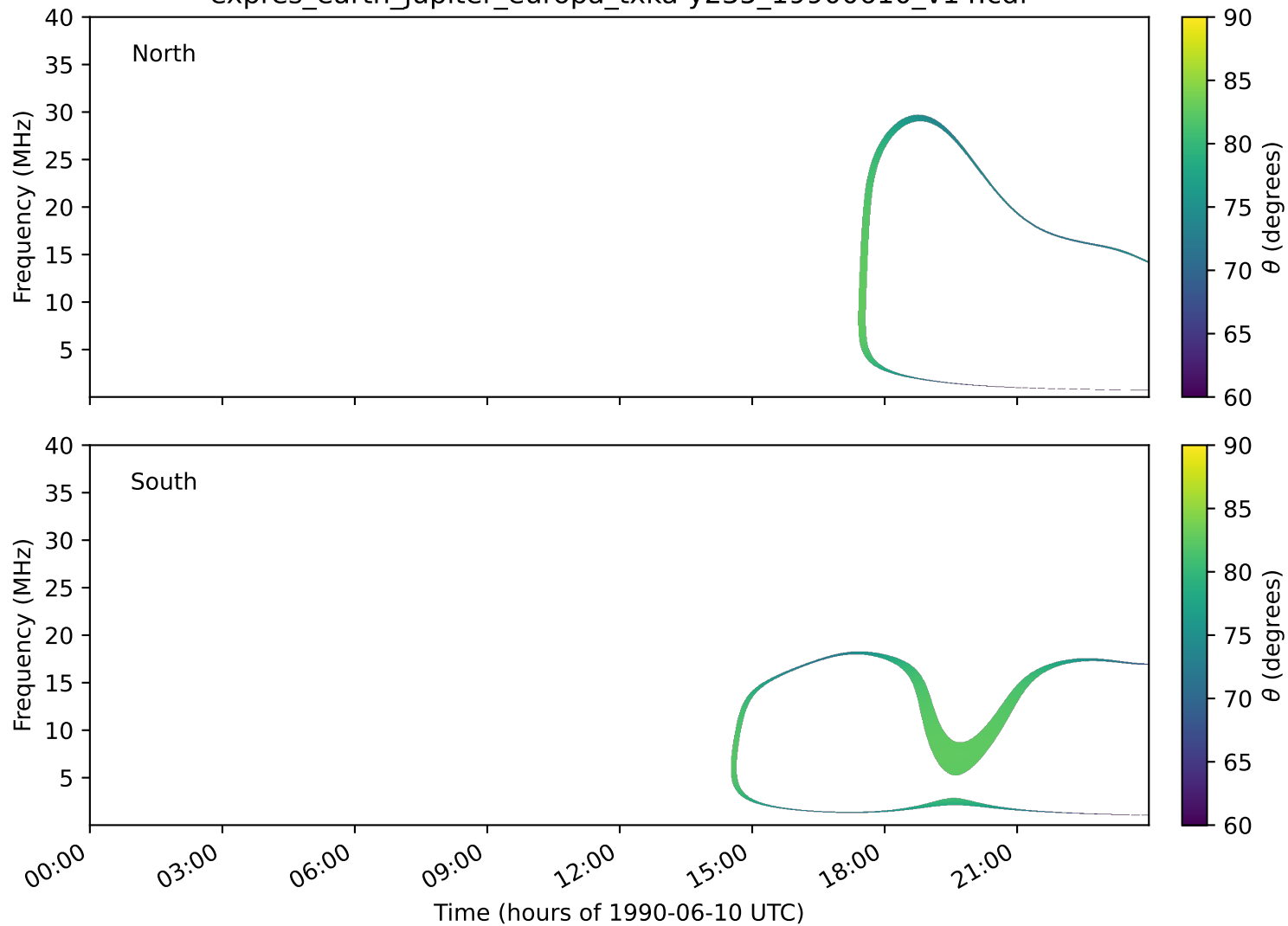
expres_earth_jupiter_europa_txka-y235_19900610_v14.cdf
