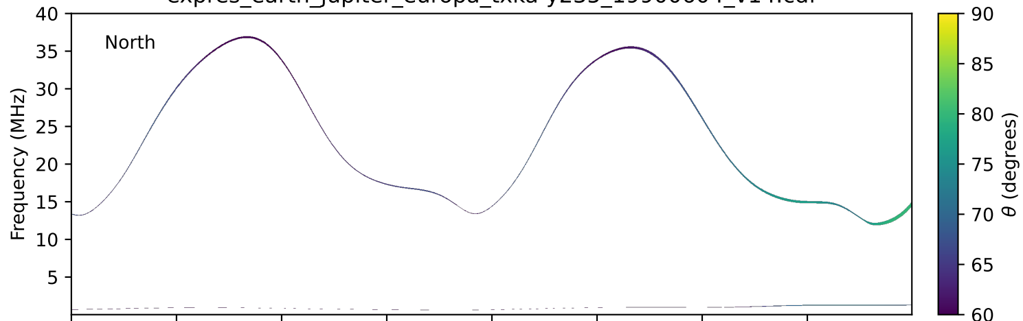
expres_earth_jupiter_europa_txka-y235_19900604_v14.cdf
