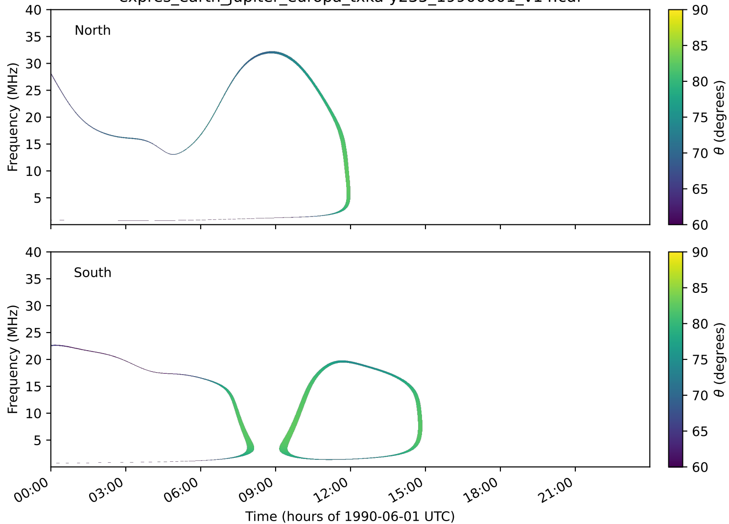
expres_earth_jupiter_europa_txka-y235_19900601_v14.cdf
