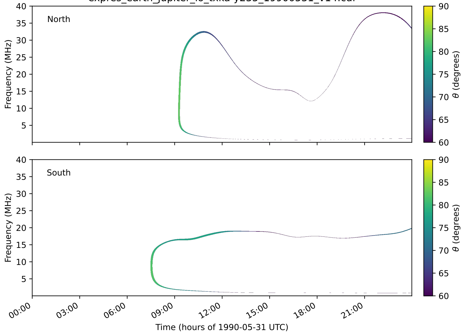
expres_earth_jupiter_io_txka-y235_19900531_v14.cdf
