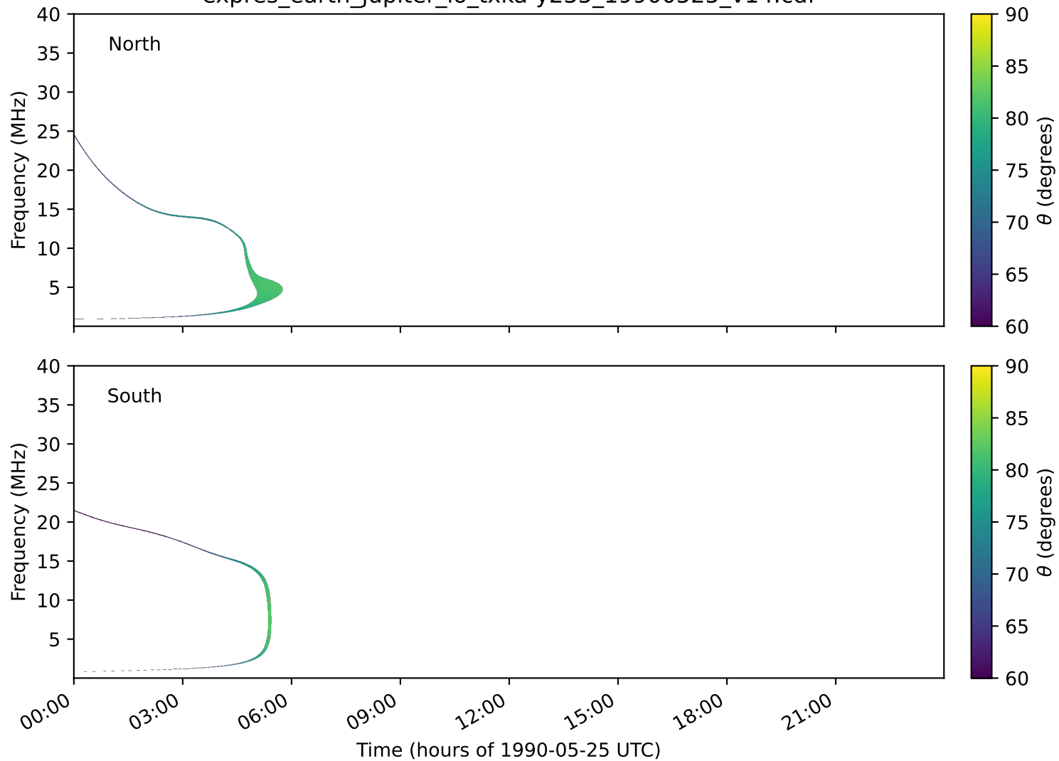
expres_earth_jupiter_io_txka-y235_19900525_v14.cdf
