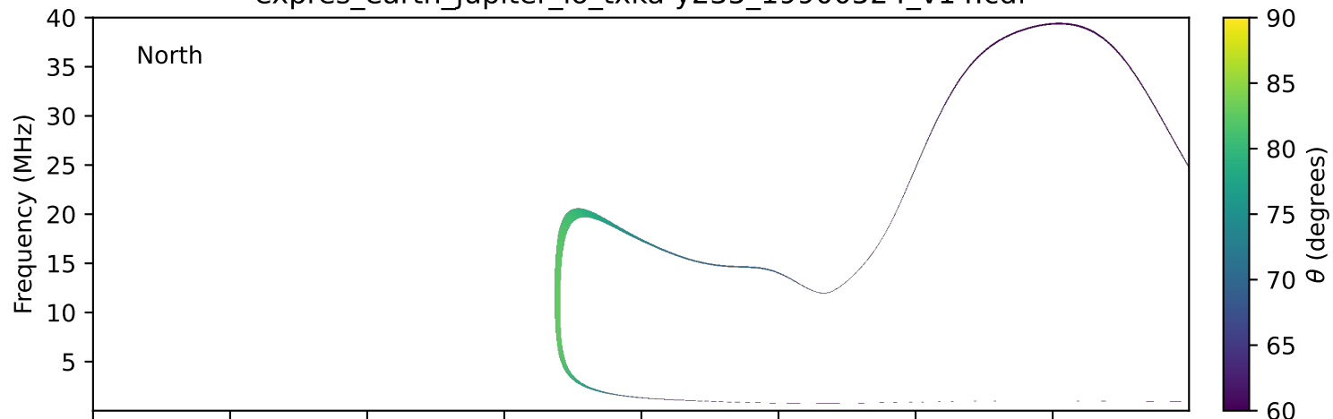
expres_earth_jupiter_io_txka-y235_19900524_v14.cdf
