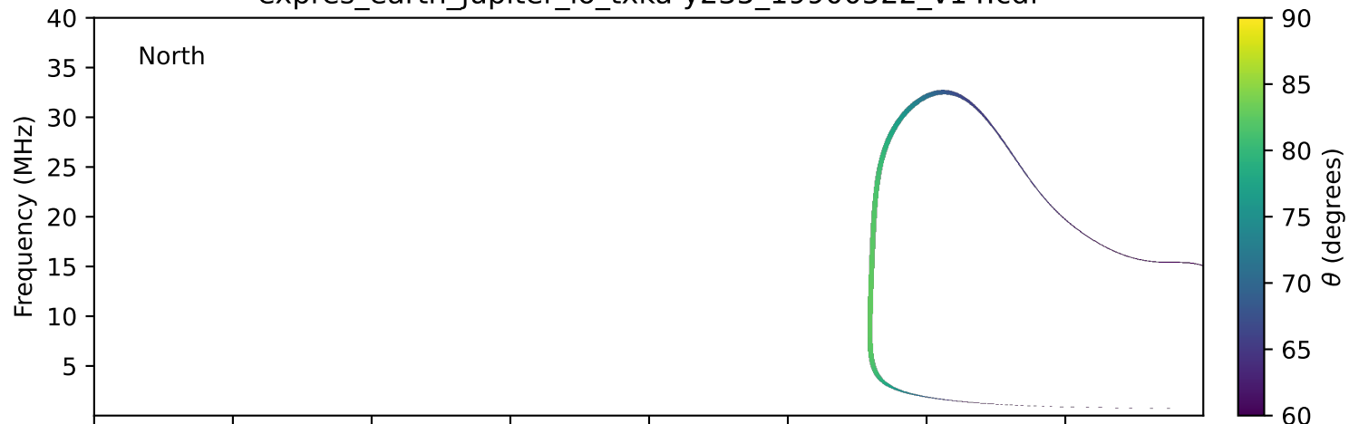
expres_earth_jupiter_io_txka-y235_19900522_v14.cdf
