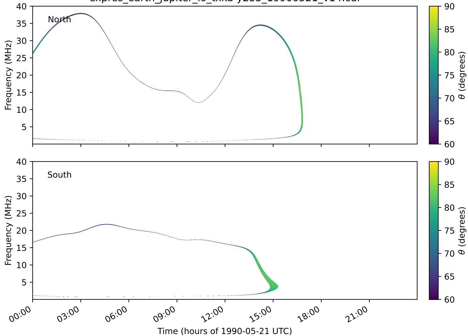
expres_earth_jupiter_io_txka-y235_19900521_v14.cdf
