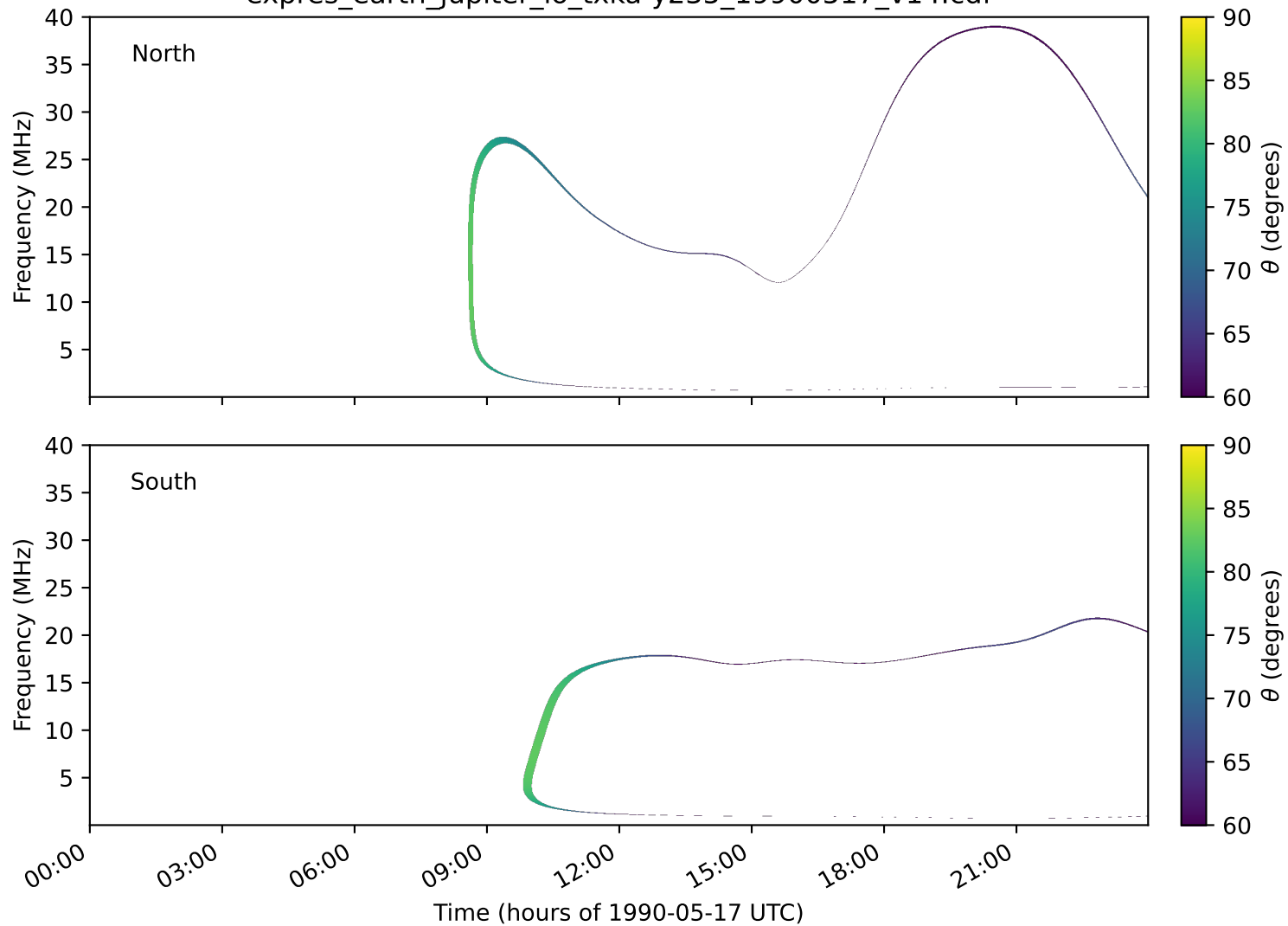
expres_earth_jupiter_io_txka-y235_19900517_v14.cdf
