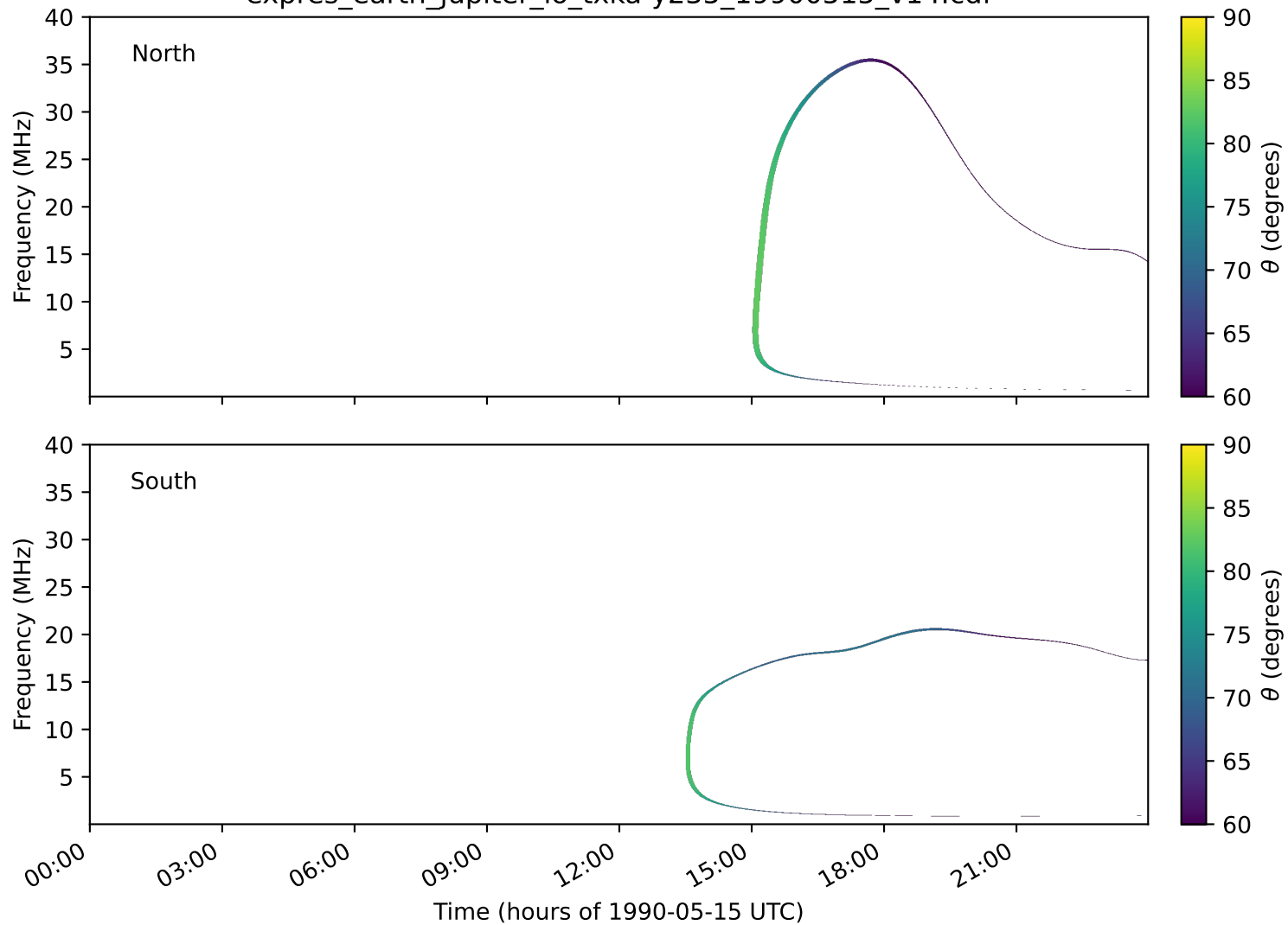
expres_earth_jupiter_io_txka-y235_19900515_v14.cdf
