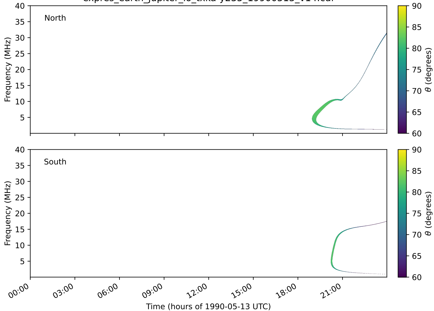
expres_earth_jupiter_io_txka-y235_19900513_v14.cdf
