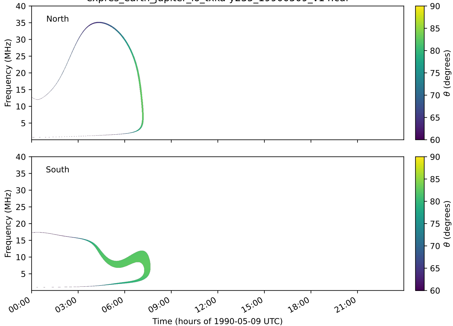
expres_earth_jupiter_io_txka-y235_19900509_v14.cdf
