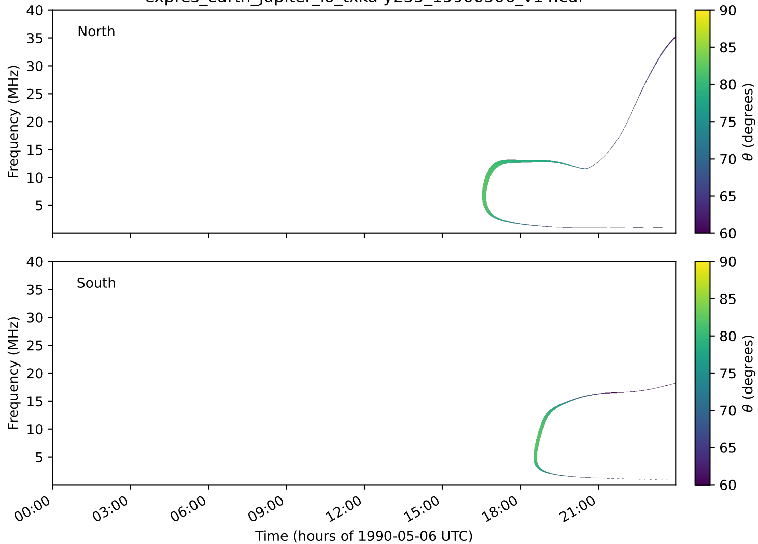
expres_earth_jupiter_io_txka-y235_19900506_v14.cdf
