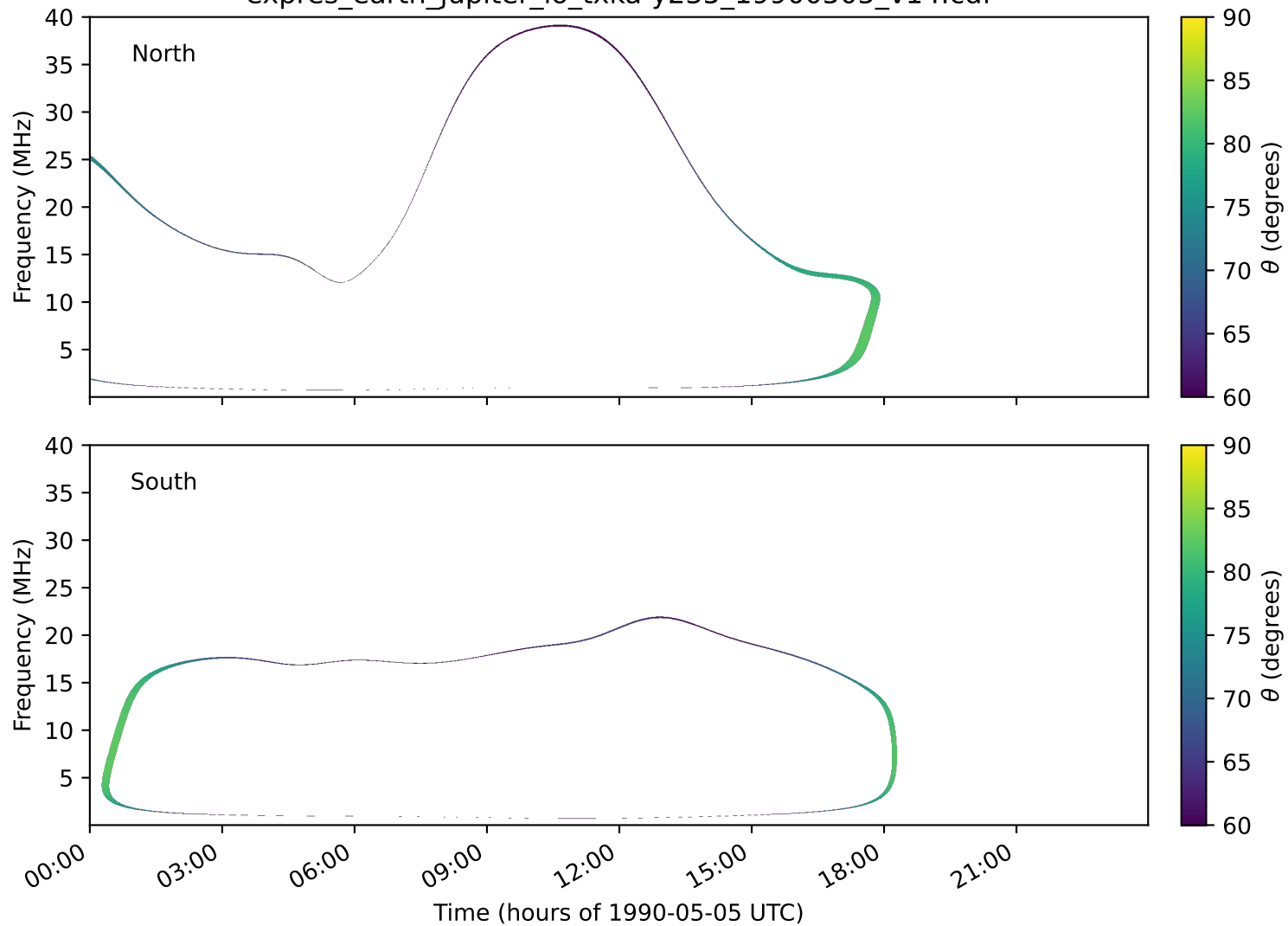
expres_earth_jupiter_io_txka-y235_19900505_v14.cdf
