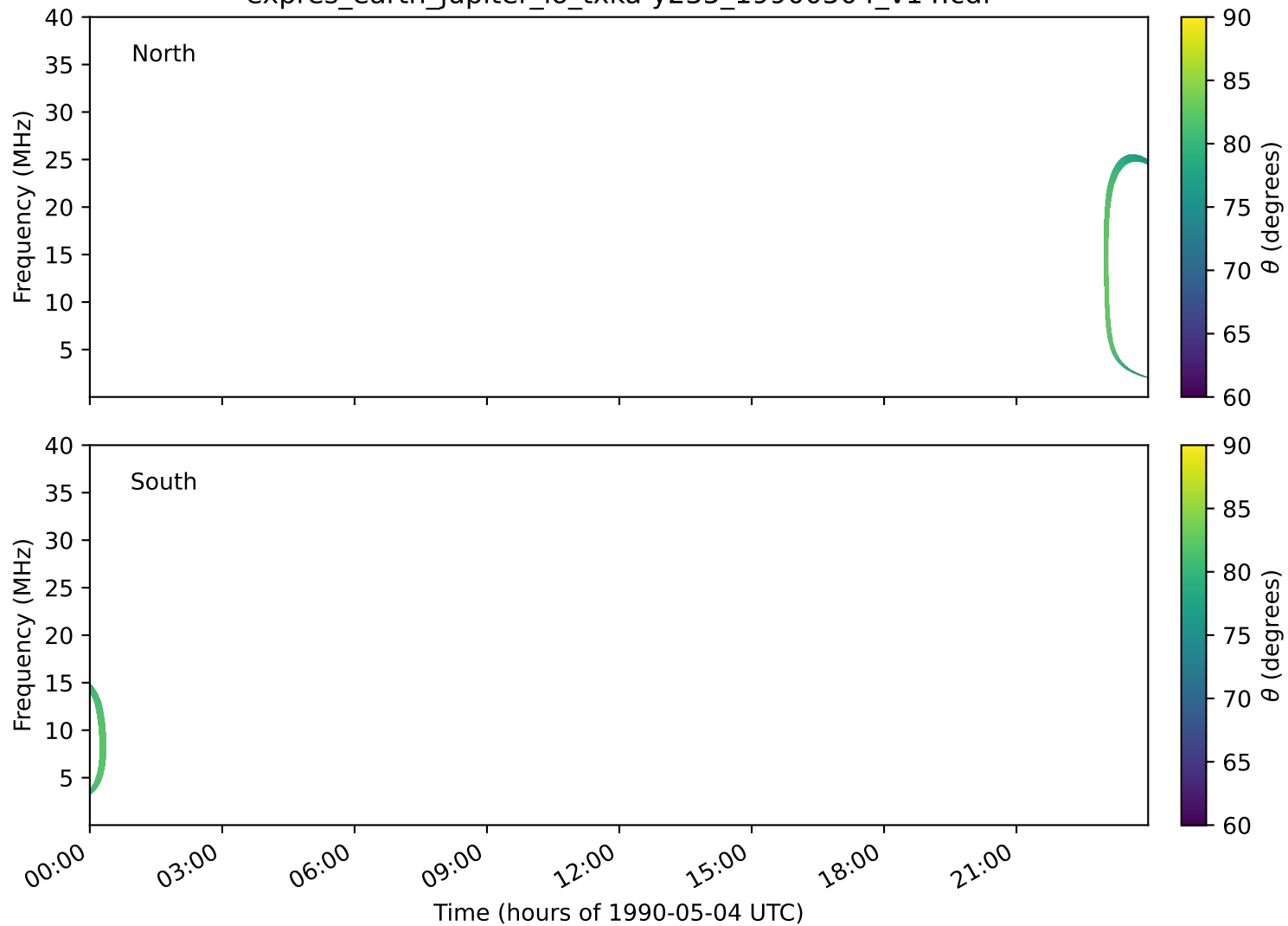
expres_earth_jupiter_io_txka-y235_19900504_v14.cdf
