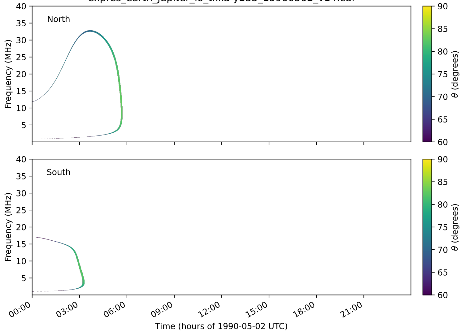
expres_earth_jupiter_io_txka-y235_19900502_v14.cdf
