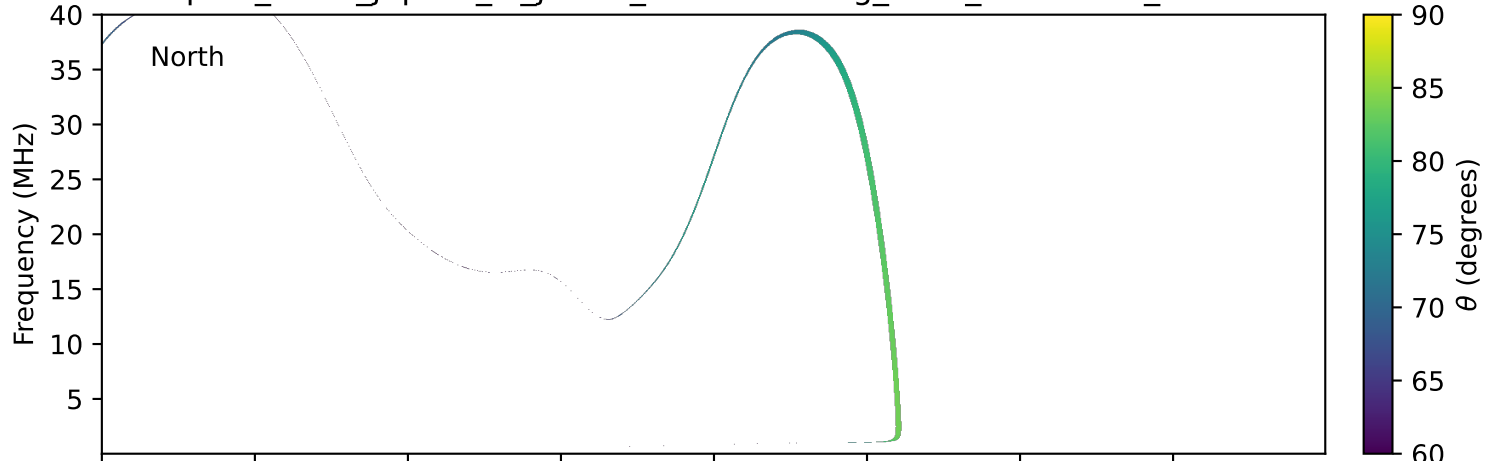
expres_earth_jupiter_io_jrm33_lossc-wid1deg_3kev_19900514_v11.cdf
