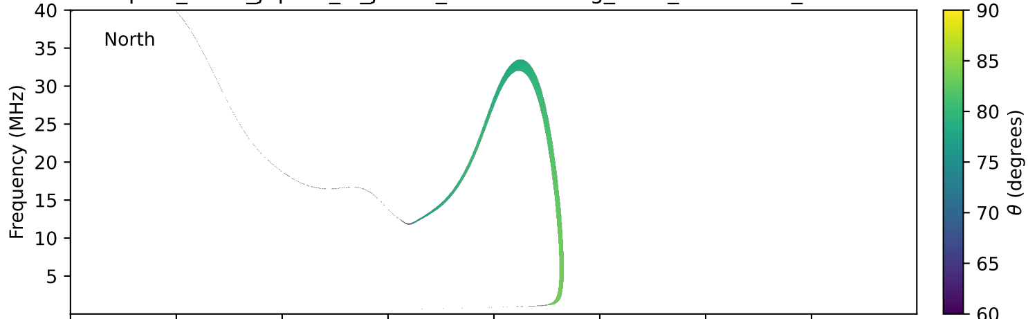
expres_earth_jupiter_io_jrm33_lossc-wid1deg_3kev_19900507_v11.cdf
