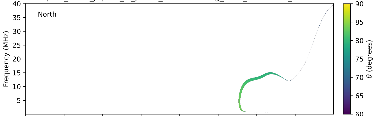
expres_earth_jupiter_io_jrm33_lossc-wid1deg_3kev_19900506_v11.cdf
