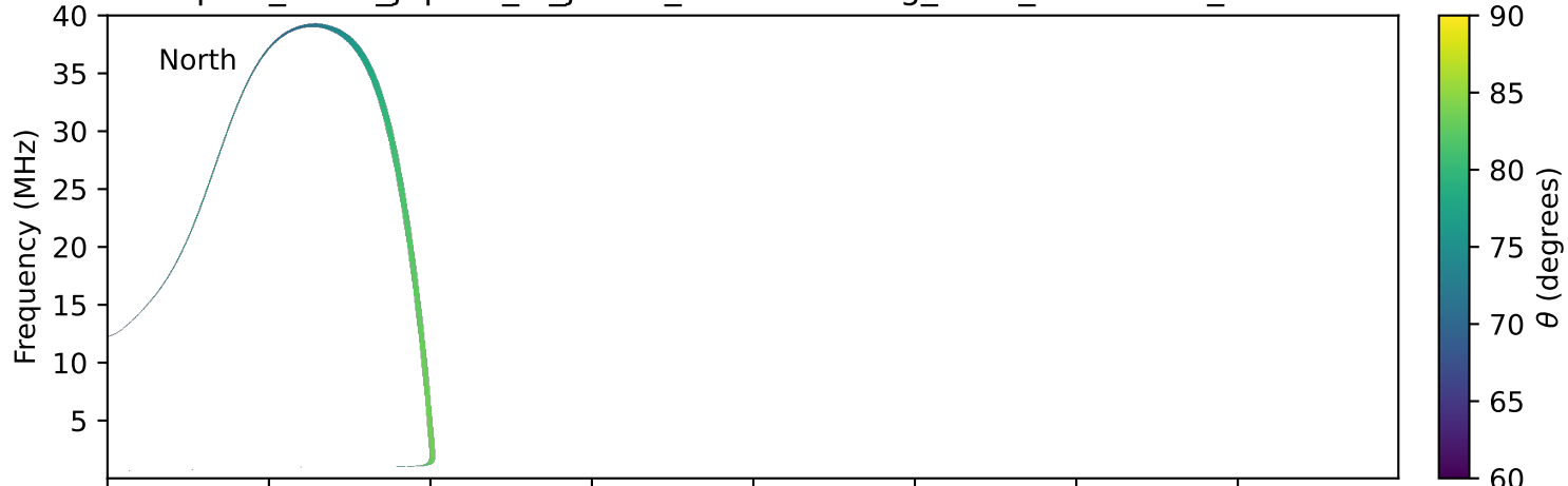
expres_earth_jupiter_io_jrm33_lossc-wid1deg_3kev_19900502_v11.cdf
