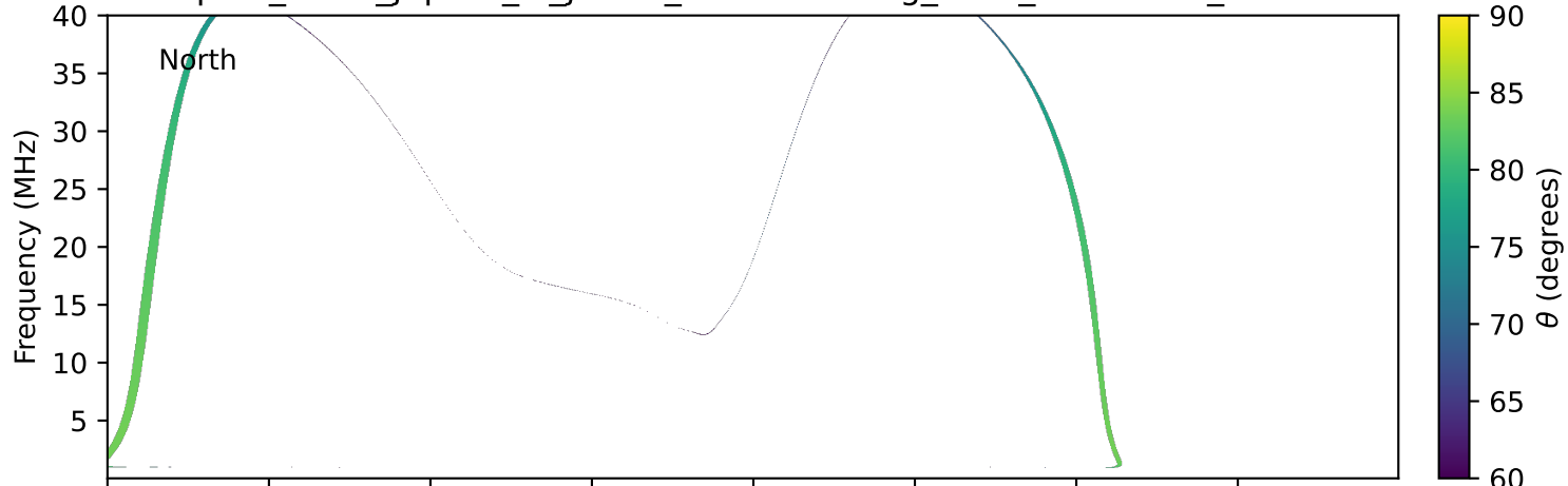
expres_earth_jupiter_io_jrm09_lossc-wid1deg_3kev_19900528_v11.cdf
