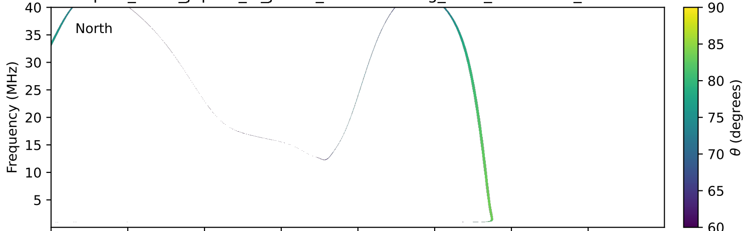
expres_earth_jupiter_io_jrm09_lossc-wid1deg_3kev_19900521_v11.cdf
