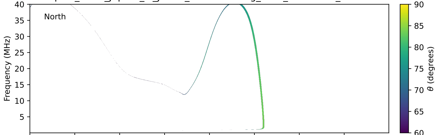
expres_earth_jupiter_io_jrm09_lossc-wid1deg_3kev_19900514_v11.cdf
