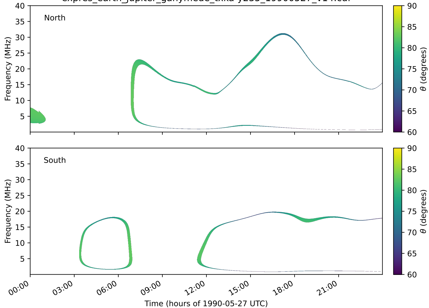
expres_earth_jupiter_ganymede_txka-y235_19900527_v14.cdf
