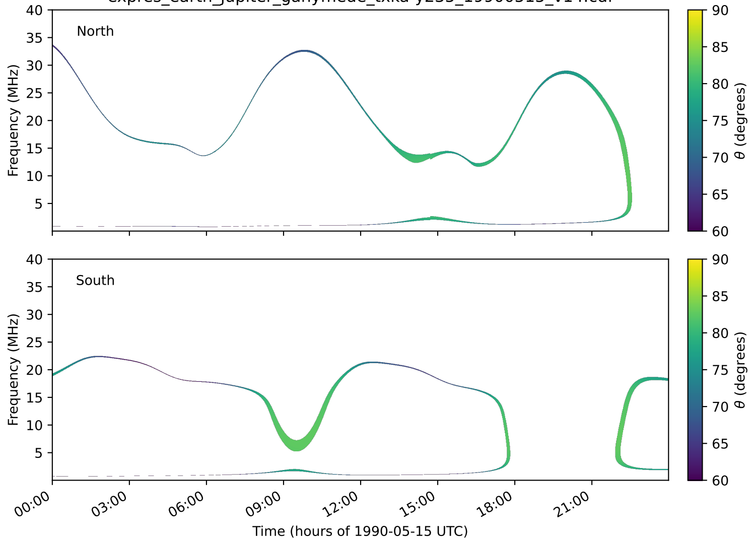
expres_earth_jupiter_ganymede_txka-y235_19900515_v14.cdf
