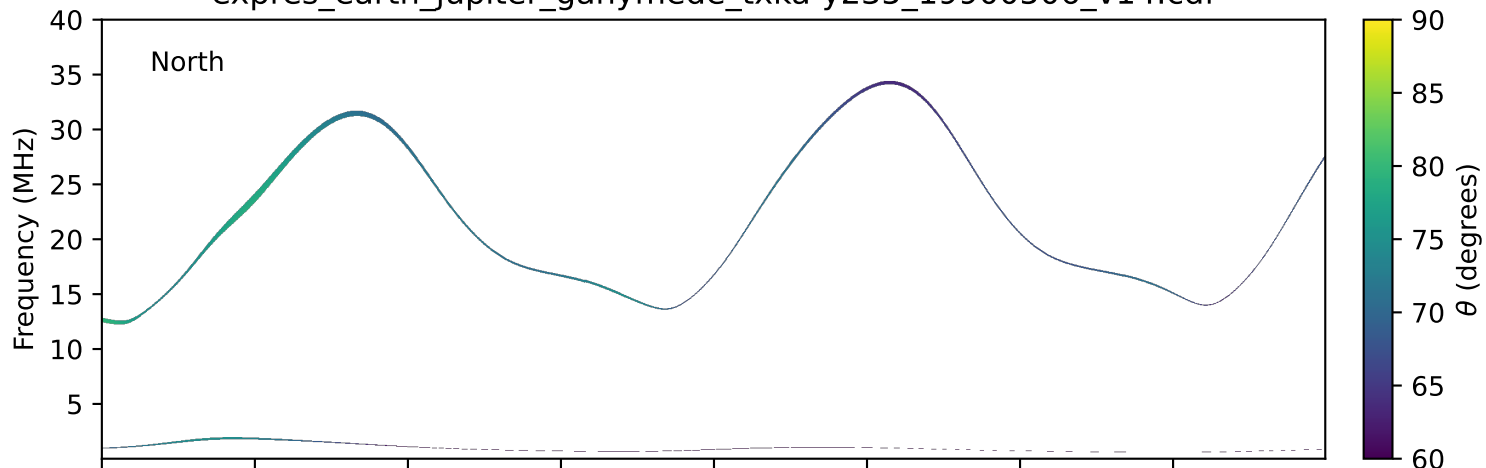
expres_earth_jupiter_ganymede_txka-y235_19900506_v14.cdf
