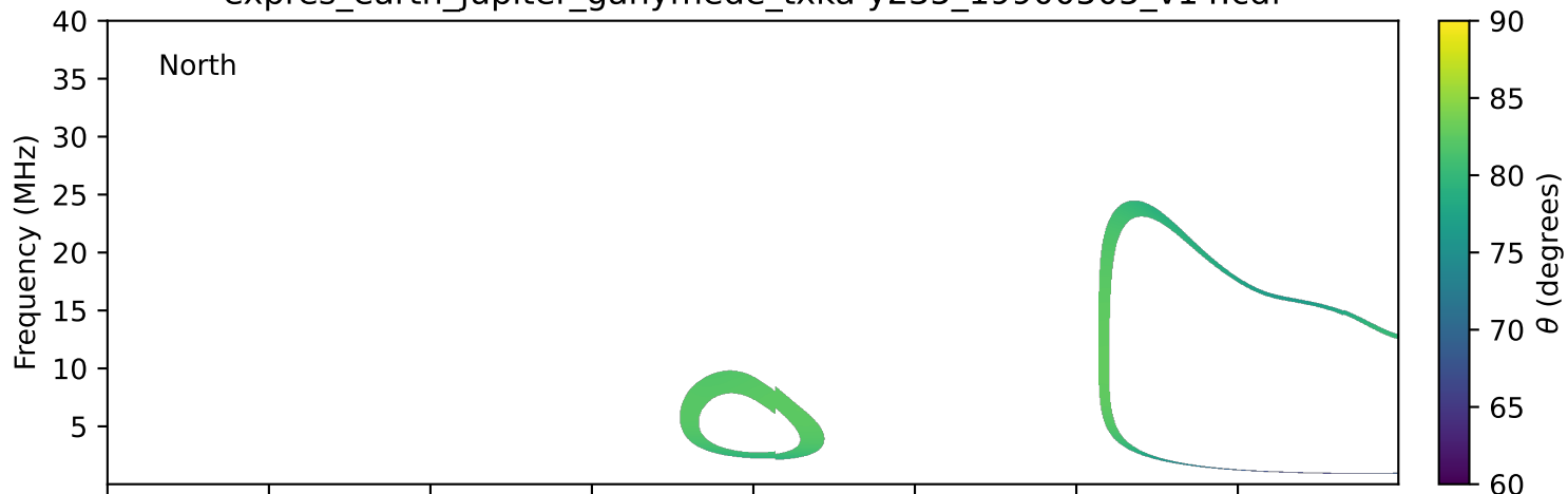
expres_earth_jupiter_ganymede_txka-y235_19900505_v14.cdf
