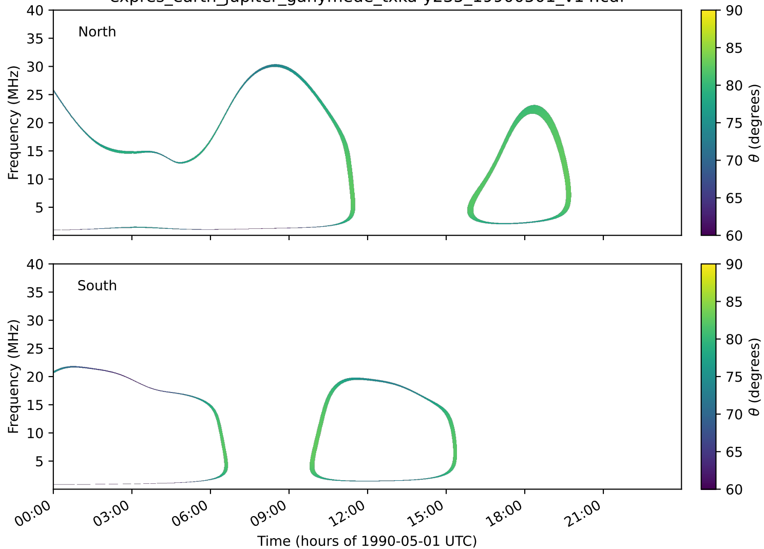
expres_earth_jupiter_ganymede_txka-y235_19900501_v14.cdf
