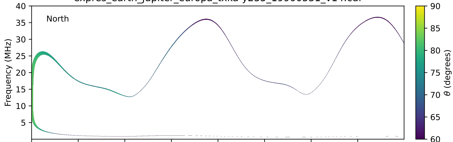
expres_earth_jupiter_europa_txka-y235_19900531_v14.cdf
