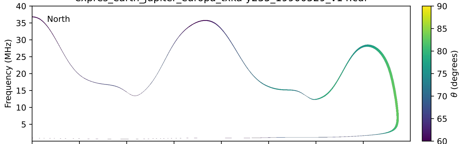
expres_earth_jupiter_europa_txka-y235_19900529_v14.cdf
