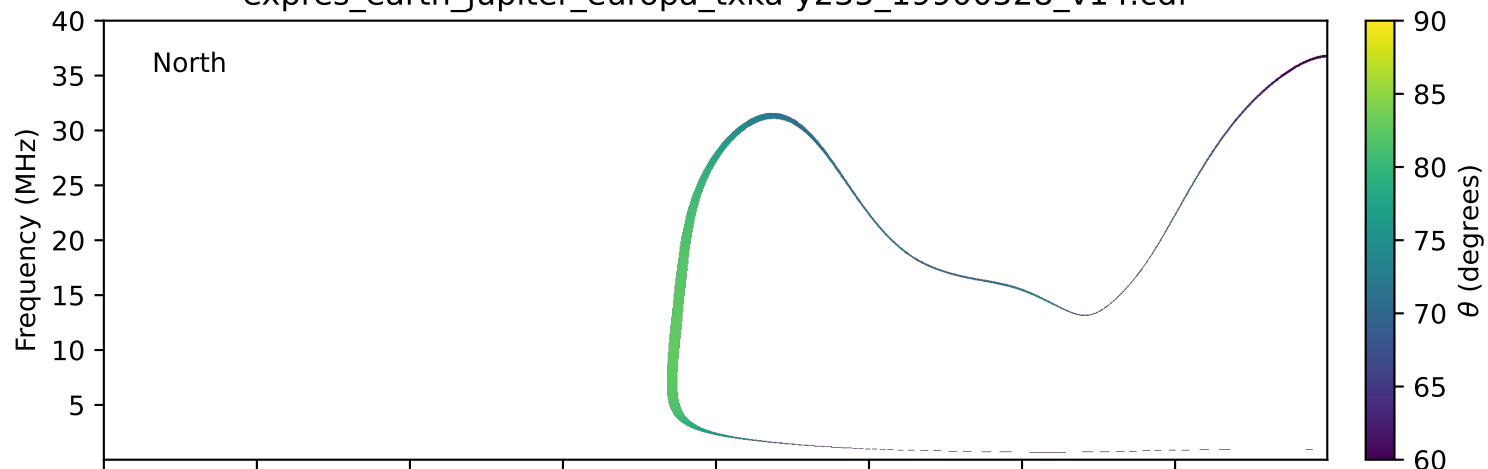
expres_earth_jupiter_europa_txka-y235_19900528_v14.cdf
