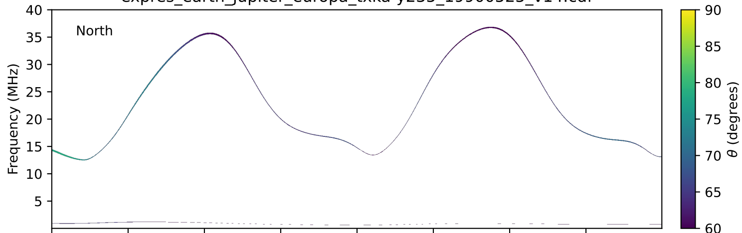
expres_earth_jupiter_europa_txka-y235_19900525_v14.cdf
