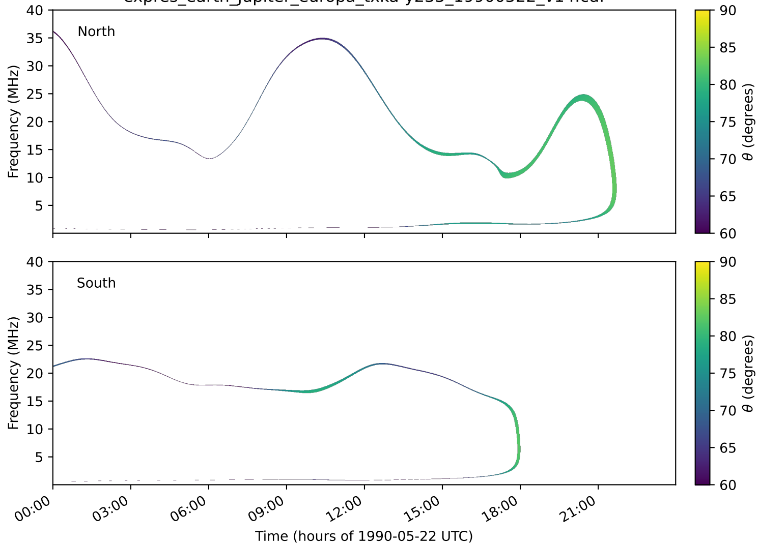
expres_earth_jupiter_europa_txka-y235_19900522_v14.cdf
