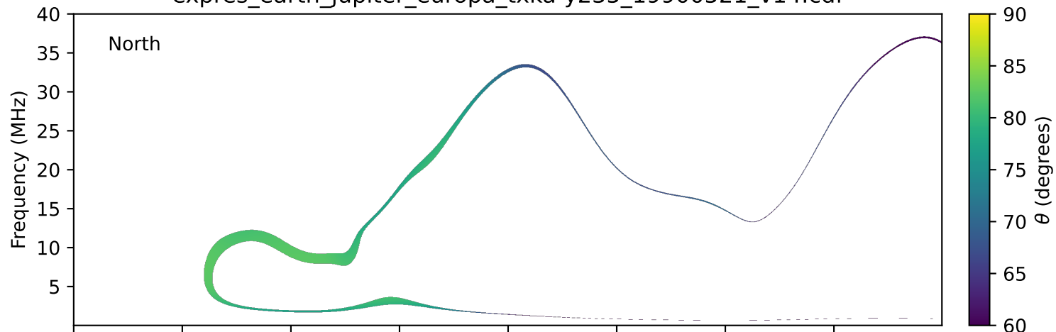
expres_earth_jupiter_europa_txka-y235_19900521_v14.cdf
