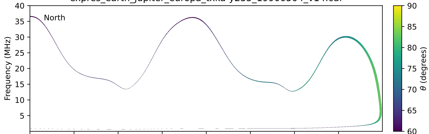
expres_earth_jupiter_europa_txka-y235_19900504_v14.cdf
