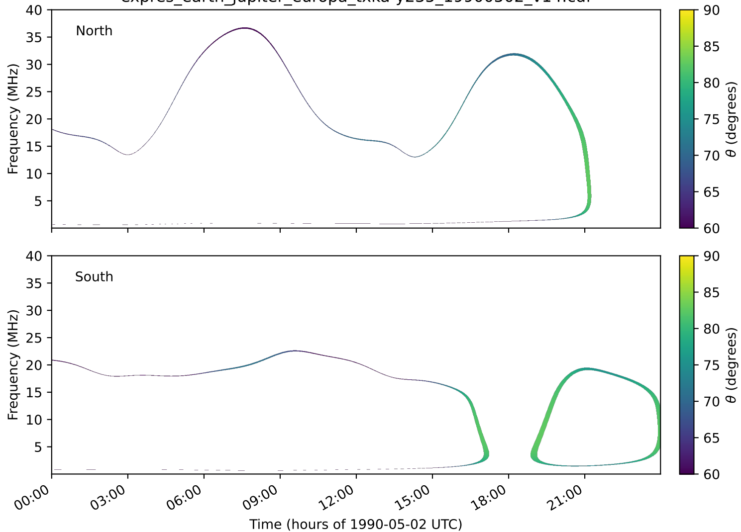
expres_earth_jupiter_europa_txka-y235_19900502_v14.cdf
