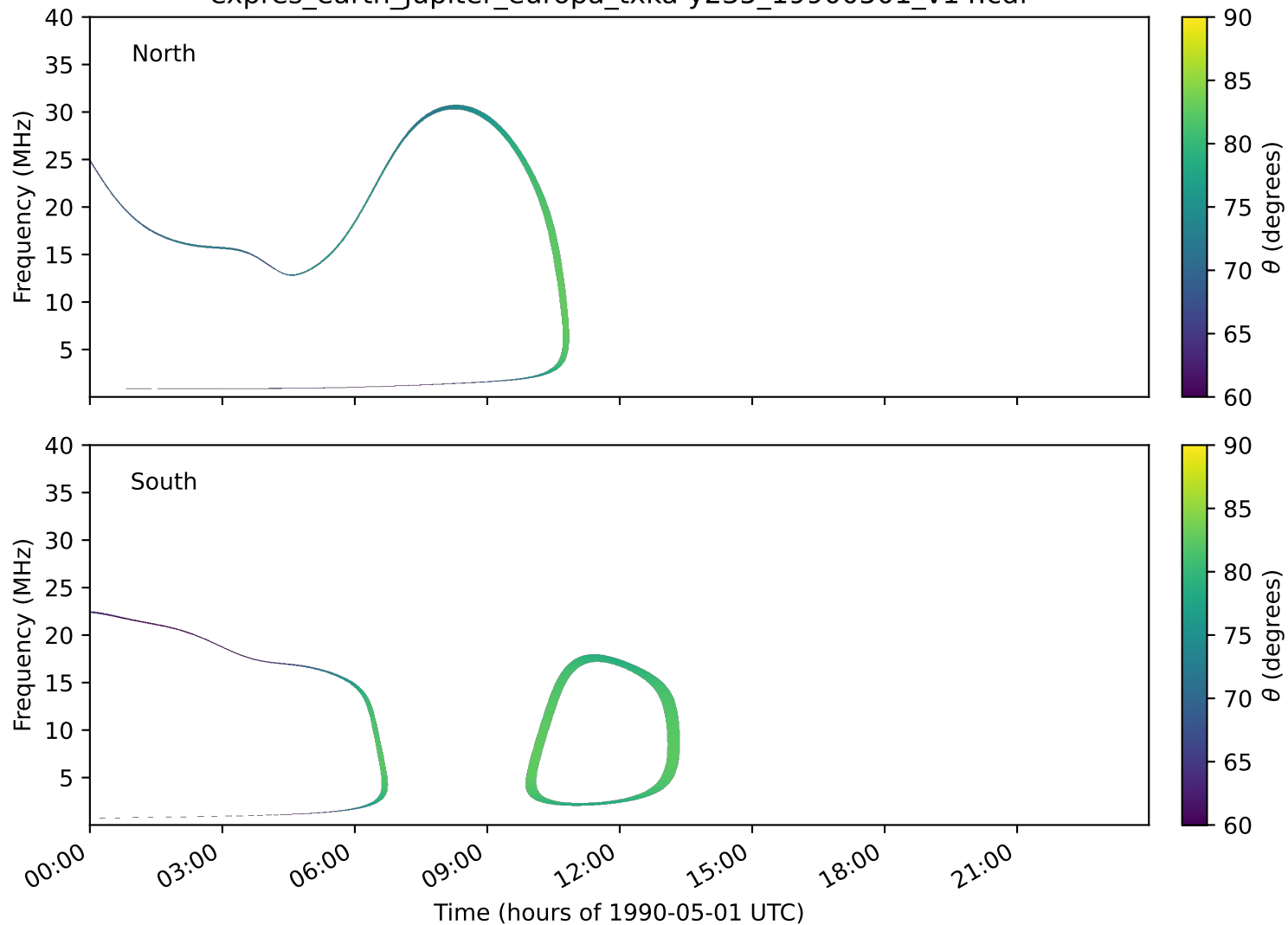
expres_earth_jupiter_europa_txka-y235_19900501_v14.cdf
