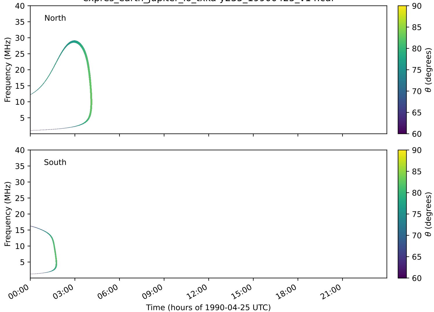
expres_earth_jupiter_io_txka-y235_19900425_v14.cdf
