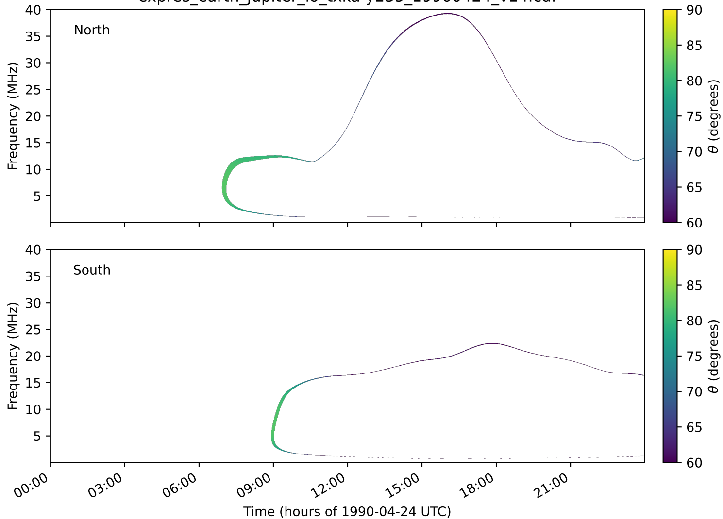
expres_earth_jupiter_io_txka-y235_19900424_v14.cdf
