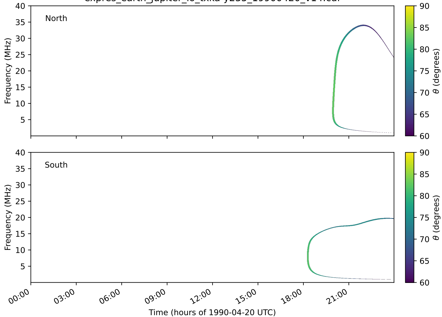
expres_earth_jupiter_io_txka-y235_19900420_v14.cdf
